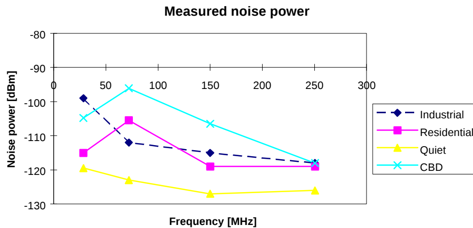
Figure 2 Average noise power measured in different environments, using the receiver with 10 kHz IF bandwidth and 500 ms measurement time
