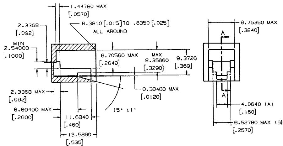
SECT. A-A
