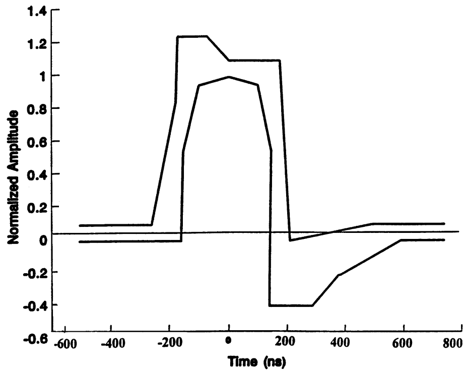
MAXIMUM CURVE
